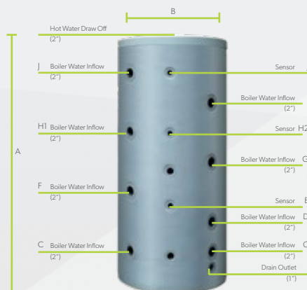
Dimensions (3000-5000L)
