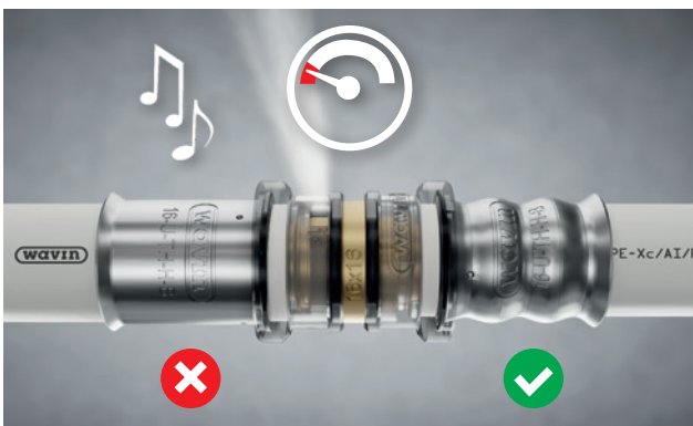
Fig. 7: ACOUSTIC LEAK ALERT. A loud whistle tone caused by the leaking air helps to trace the unpressed fitting.
