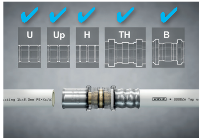
Fig. 5: MULTIJAW. Pressing possible with the most common pressing profiles. Wavin System Warranty.
