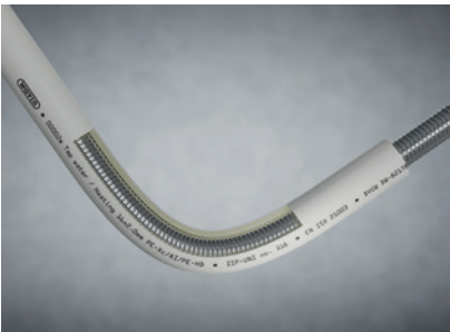
Fig. 23: Bending the pipe with a bending spring.
