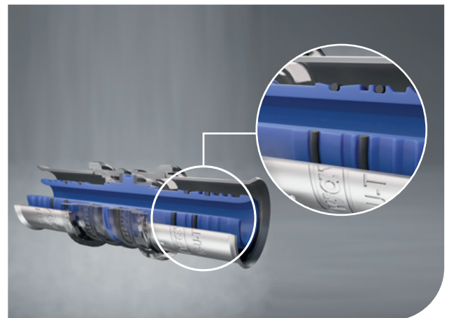
Fig.11: ULTRASEAL O-rings have been tested even beyond the ISO requirements for life test simulation.
