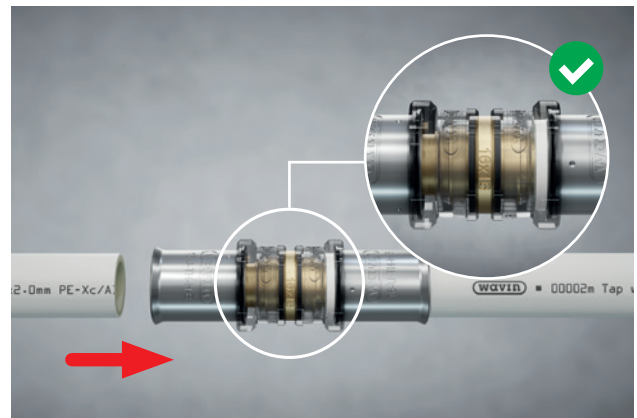
Fig.8: IN4SURE™ helps to check if the pipe is inserted properly.
