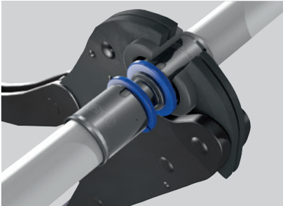
Fig. 22: Positioning the pressing jaws on the fitting with Tigris K1 and Tigris M1.
