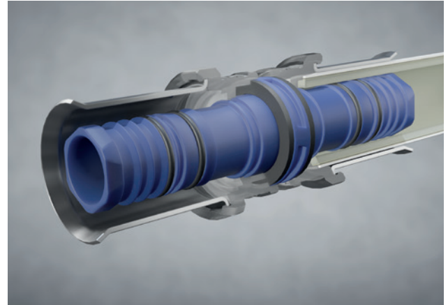
Fig.10: EASYFIT pipe insertion without calibration.
