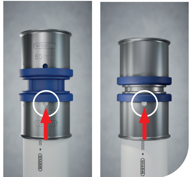
Fig. 13: IN4SURE™ helps to check if the pipe is inserted properly.
