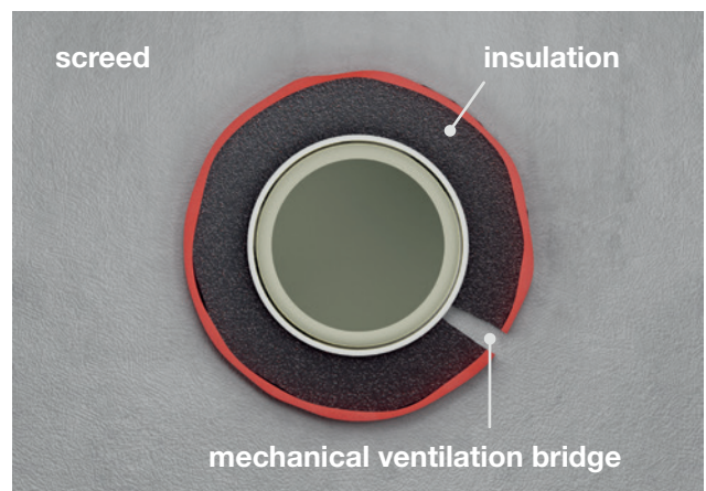
Fig 35: Mechanical vibration transmission through defective pipe insulation.
