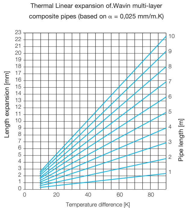
Fig. 30: Thermal Linear expansion.
