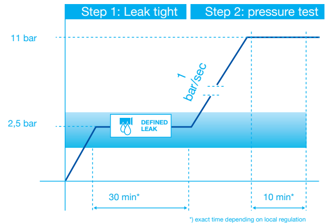
Fig. 26: Pressure test protocol when testing with water.
