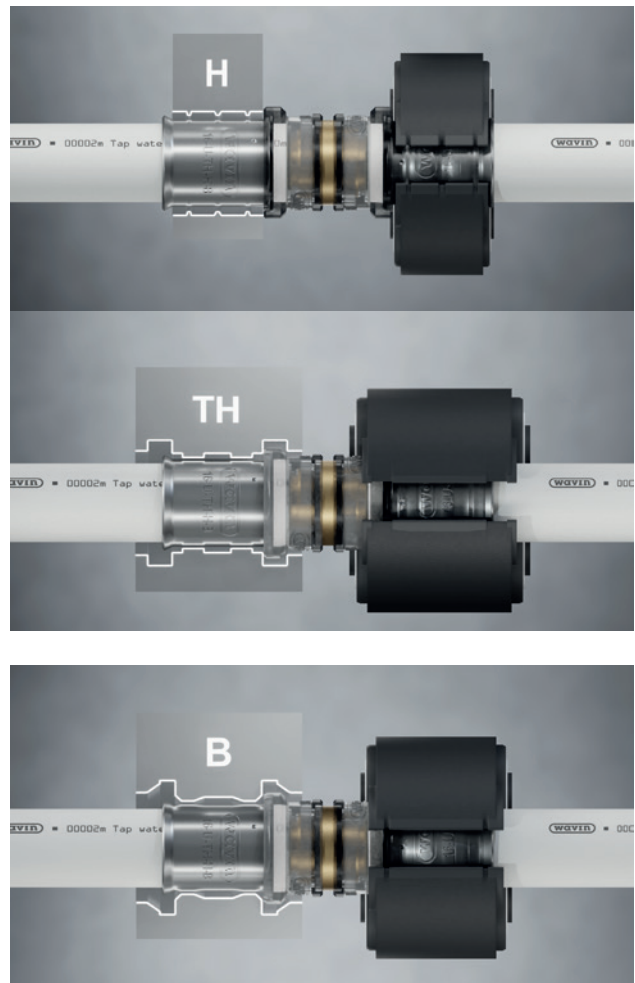
Fig. 37: Released pressing profiles for Tigris K5, Tigris M5.
