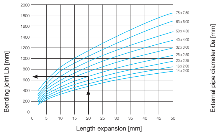
Fig. 32: Bending joint classification of Wavin multi-layer composite pipes.
