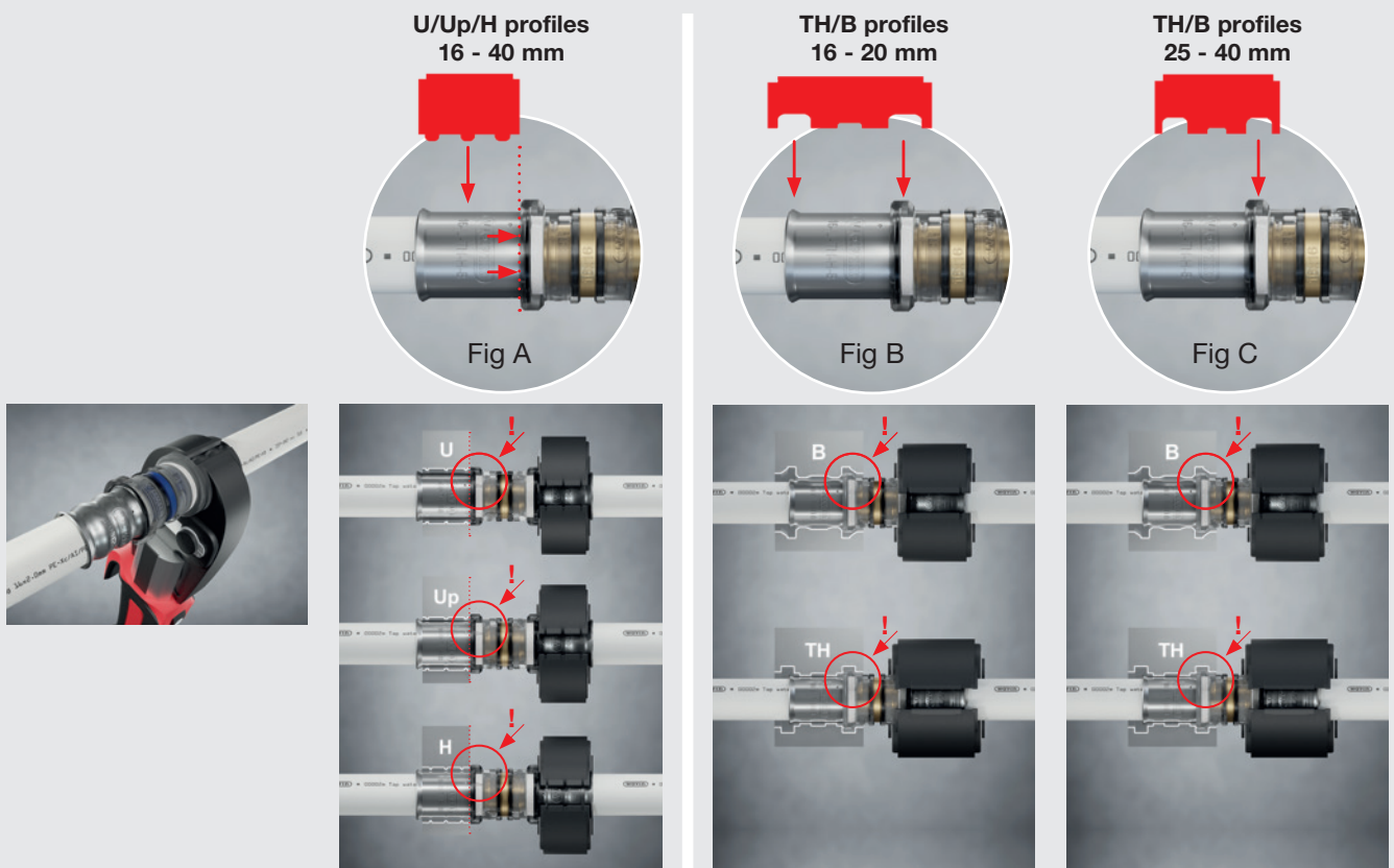
Fig. 21: Positioning the pressing jaws on the fitting with Tigris K5 and Tigris M5.
