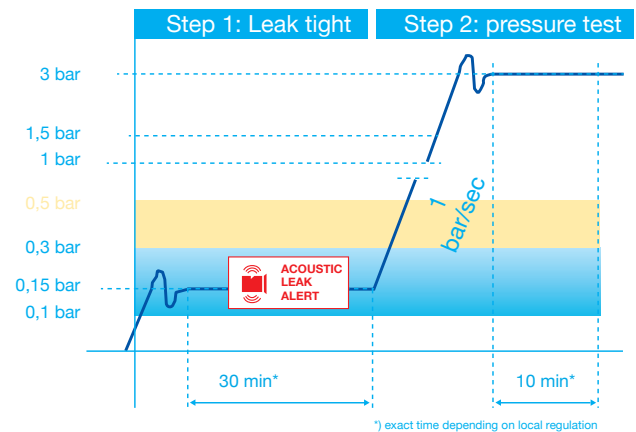
Fig. 28: Pressure test protocol when testing with air.
