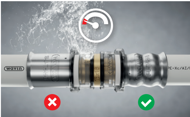
Fig. 6: DEFINED LEAK in the pressure test reveals with leaking water the unpressed fitting.
