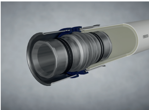
Fig. 15: Low insertion force thanks to the patented hexagonal sleeve-end.
