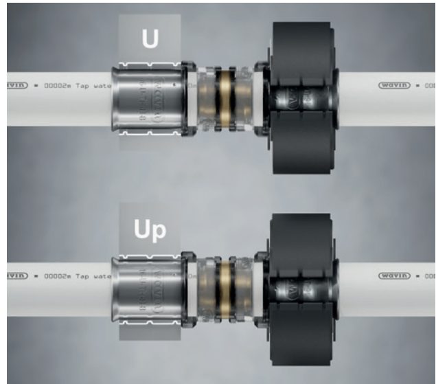
Fig. 36: Released pressing profiles for Tigris K1/K5, Tigris M1/M5.
