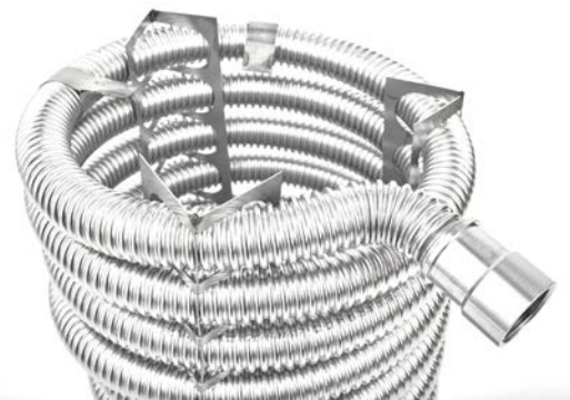
Special heat pump coil
